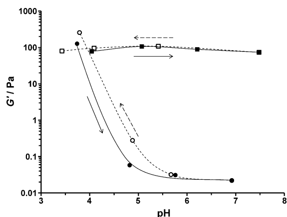
Figure 4. Variation in gel storage modulus ( G' ) for a 10% w/w HOOC-PGMA 56 -PHPMA 155 diblock copolymer worm/sphere dispersion at 25 °C during a pH switch from 3.7 to 6.9 (filled circles), followed by a switch back to pH 3.8 (open circles). As a control experiment, a gel composed of H 3 COOC-PGMA 59 -PHPMA 160 diblock copolymer worms showed essentially no change in the storage modulus, G' , from pH 3.4 to 7.5 (open and filled squares). The solid lines represent increasing pH, while the dotted lines represent decreasing pH.
